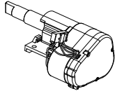
1289474-SP Top Cove Gear Box Installation Asm
