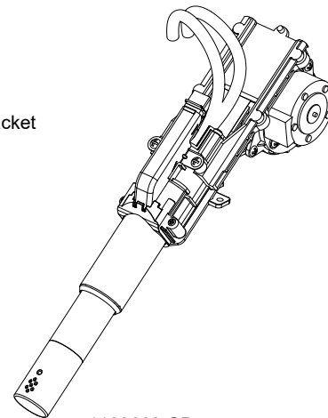
1183663-SP Nozzle ASM
